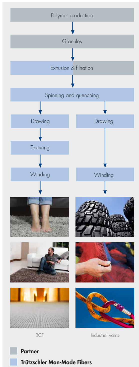
Filament processes
