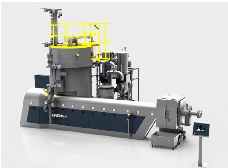
VACUREMA® Basic with vacuum reactor, extruder and filter
