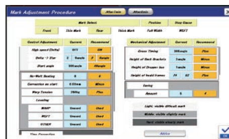
Adjustment Support – Corrective actions for stop marks (list)
