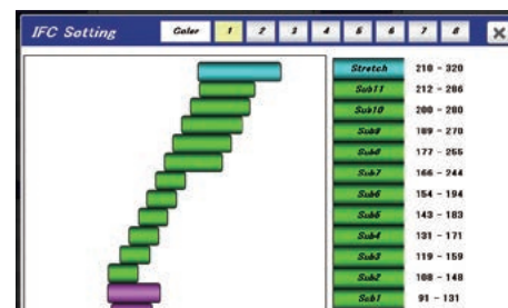
Adjustment Support – Corrective actions for weft faults (Intelligent Filling Controller (IFC))
