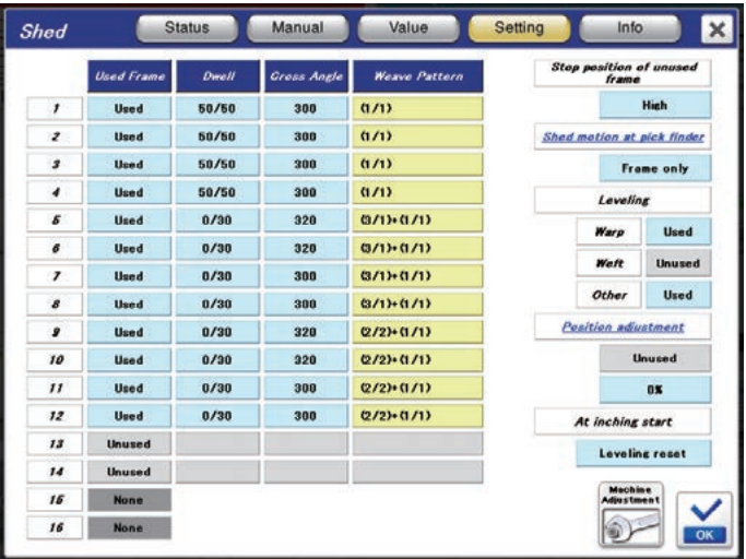
Dwell angle, cross-timing selection screen
