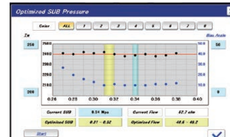
Adjustment Support – Optimization of sub pressure (Intelligent Air-Saving System (IAS))*
