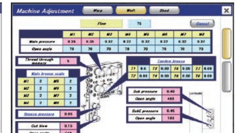
Mechanical adjustment – Weft insertion
